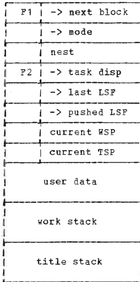
A Local Stack Frame
